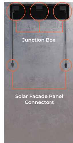
BACK VIEW
