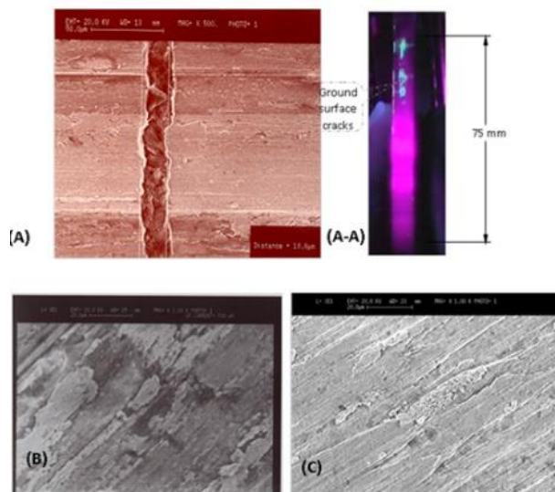
Figure 7 - Ground surface behaviour for Triboloy T800 at settings: A) Pre-set force in the disc spring is 1300N; B) Pre-set force in the disc spring is 650 N; C) Pre-set force in the disc spring is 520 N
