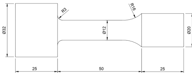
Figure 1 - Test specimen
