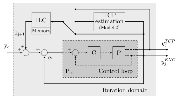
Figure 13 - Block diagram for the ILC for path planning containing three different feedback possibilities: (1) feedback from the encoder signal directly, (2) feedback from an estimation of the TCP out of model 2 and the encoder signal (3) feedback from direct measurement of the TCP with an external cross grid [22]
