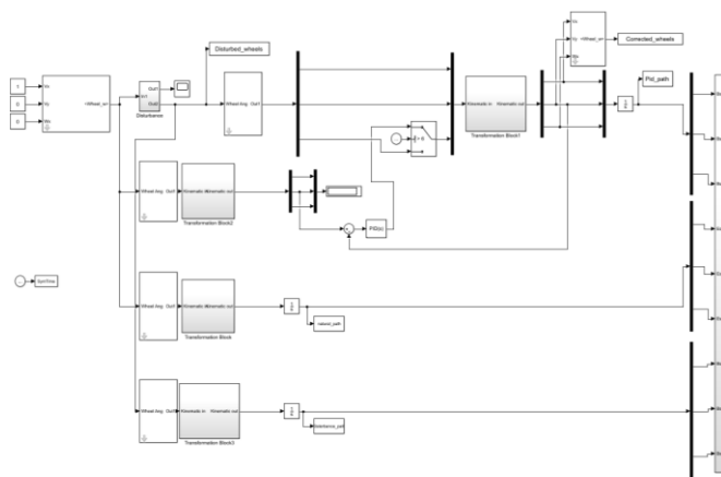
Figure 9 – Simulink Model of AGV
