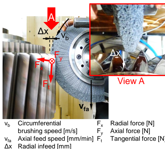
Figure 2 - Experimental setup
