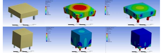
Figure 12 - FEM displacements.
