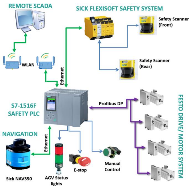
Figure 7 – Integrated electronic system
