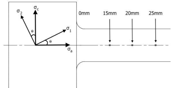
Figure 2 - XRD measurement locations and principle stress orientation
