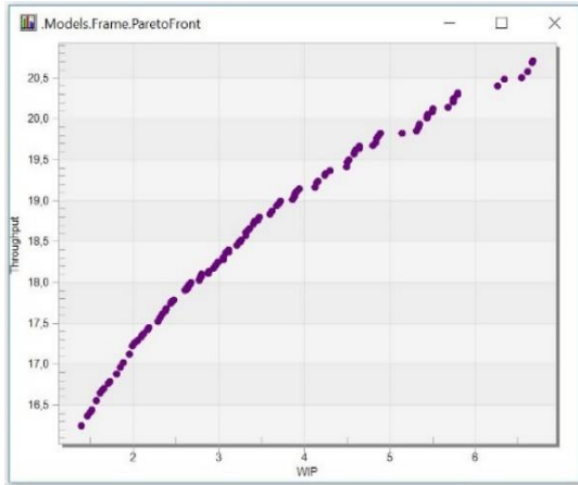
Figure 3 - Phase one results obtained by MOOSolver presented as a Pareto front in the DES product
