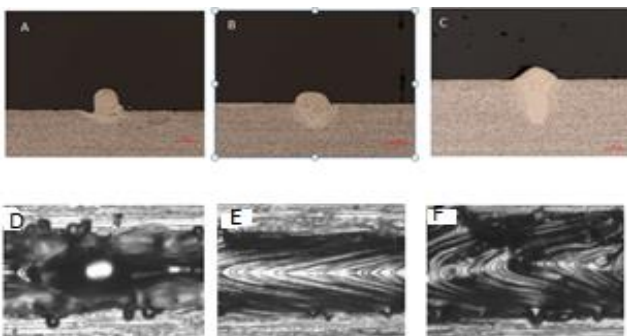
Figure 1 - Cross-sectional and top views of Ti6Al DMLS single tracks on a substrate
