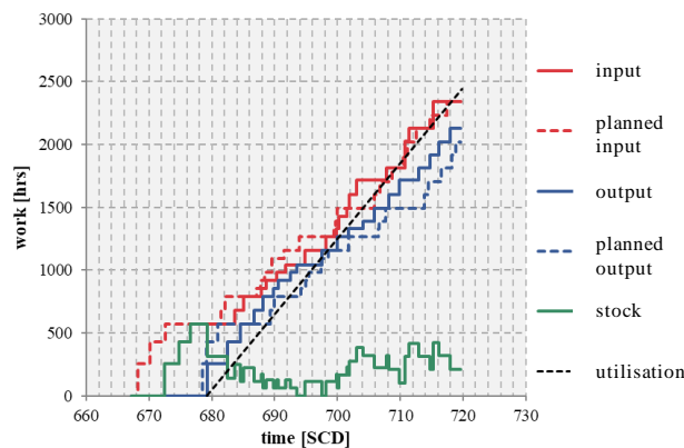
Figure 2 - Throughput Diagram
