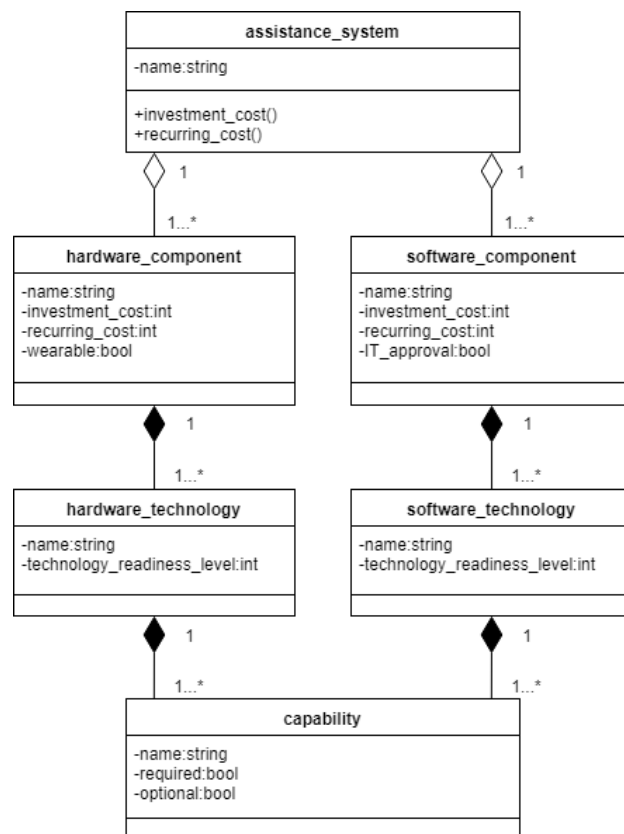
Figure 1 - UML diagram of the cognitive assistance system structure model
