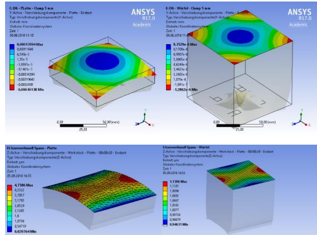
Figure 13 - Pin (top) vs. conventional (bottom) clamping FEM.
