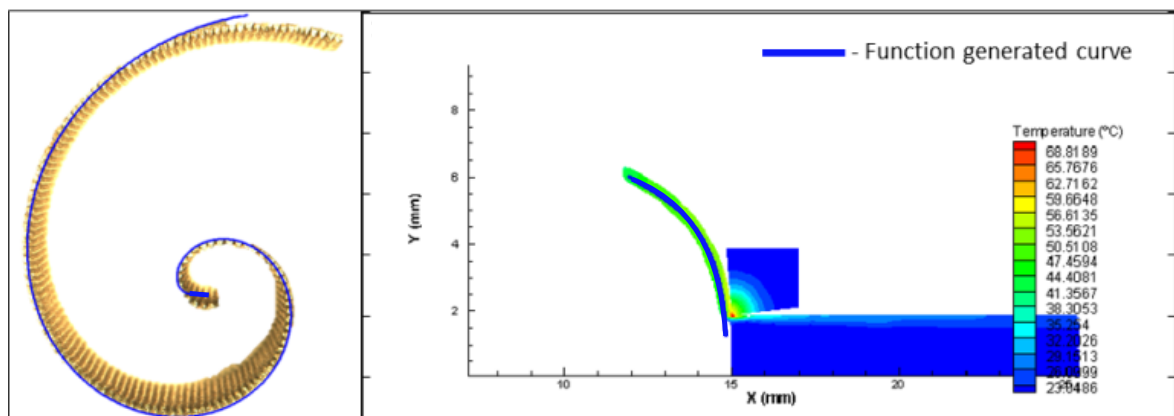
Simulated : \varphi_c = 2.975
