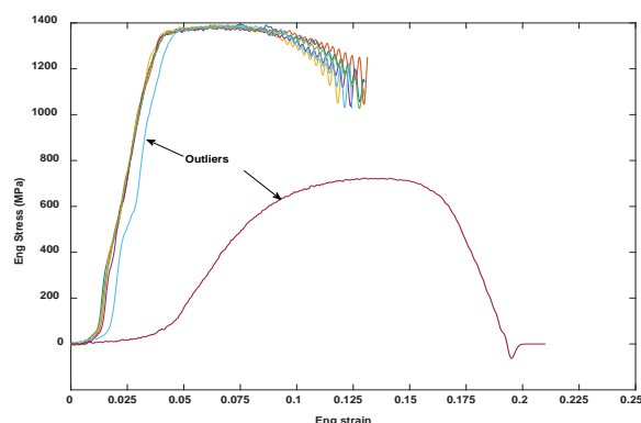
Figure 3 - Stress-strain curves for the seven AB specimens that were tested at an average strain rate of 250 \text{ s}^{-1} .
