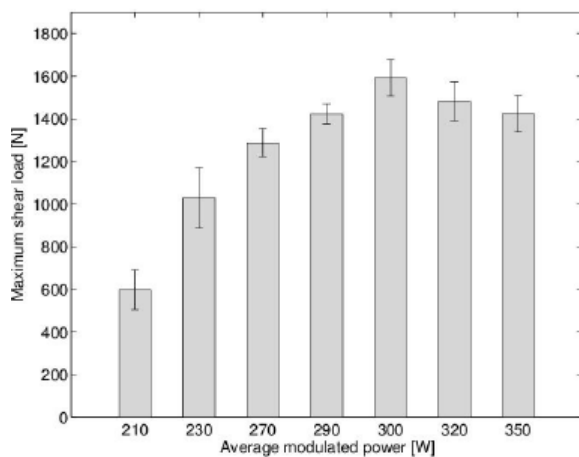
Figure 5 - Shear loads with different average powers [5]
