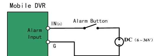
Fig 2.11 Alarm Input Connection
