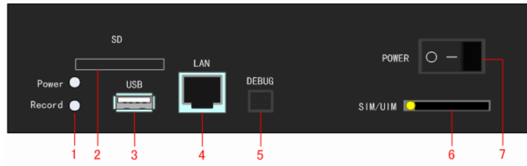
Fig 2.1 DS-8104HMI-M front panel
