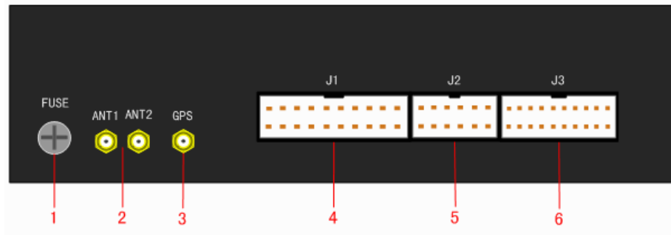
Fig 2.2 DS-8104HMI-M rear panel
