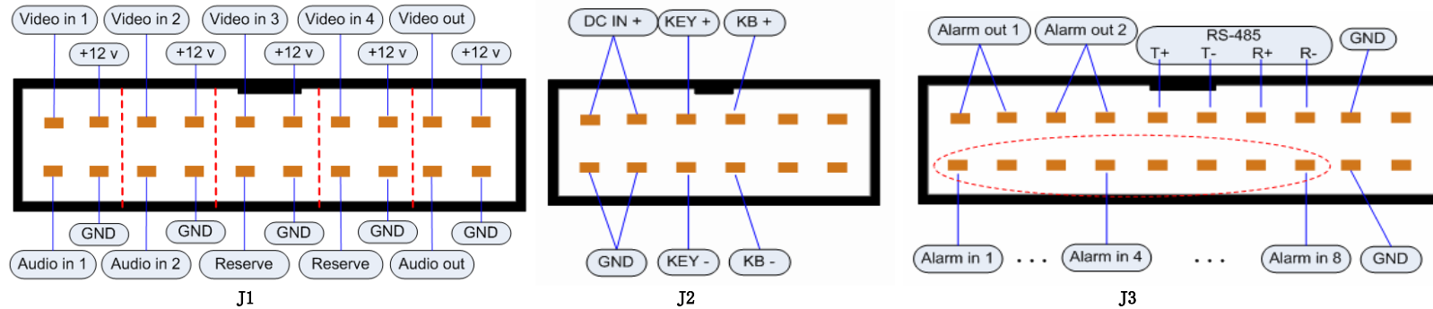
Fig 2.3 J1, J2 and J3 interfaces
