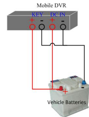
Fig 2.10 KEY connect with vehicle batteries
