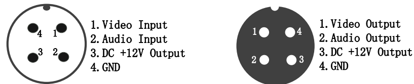
Fig 2.4 Aviation connector definition (Left side is input channel, 4 male connectors; right side is output channel, 1 female connector.)
